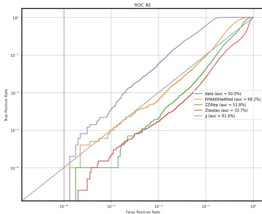
Weighted Training (capped weights)
