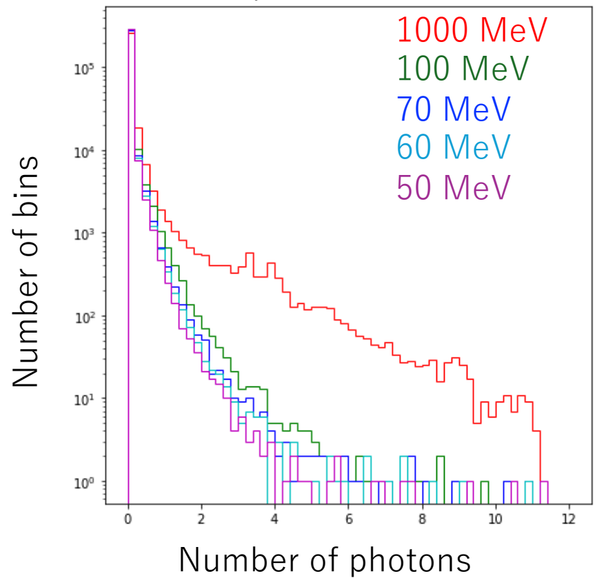
Number of photon distribution for bins
