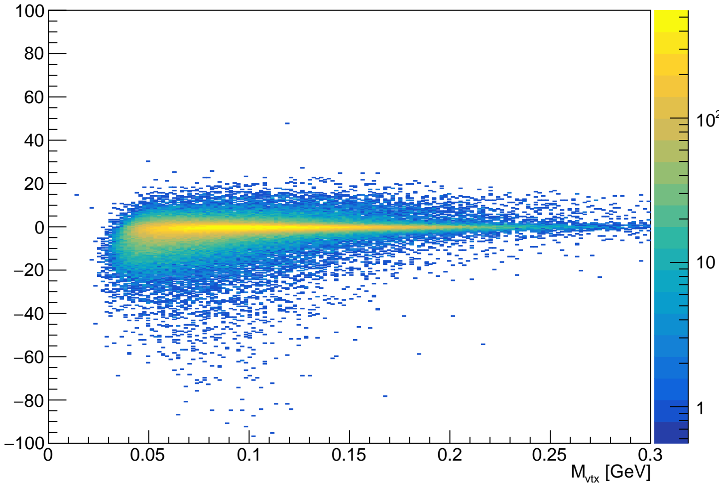
tridentL1L1-BothClusters_vtx_InvM_vtx_z_hh
