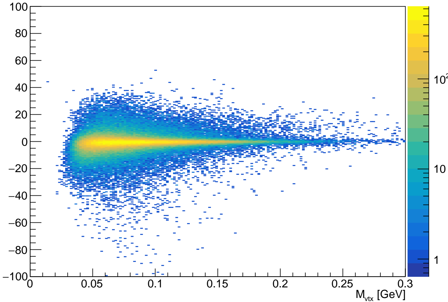
tridentL1L2-BothClusters_vtx_InvM_vtx_z_hh
