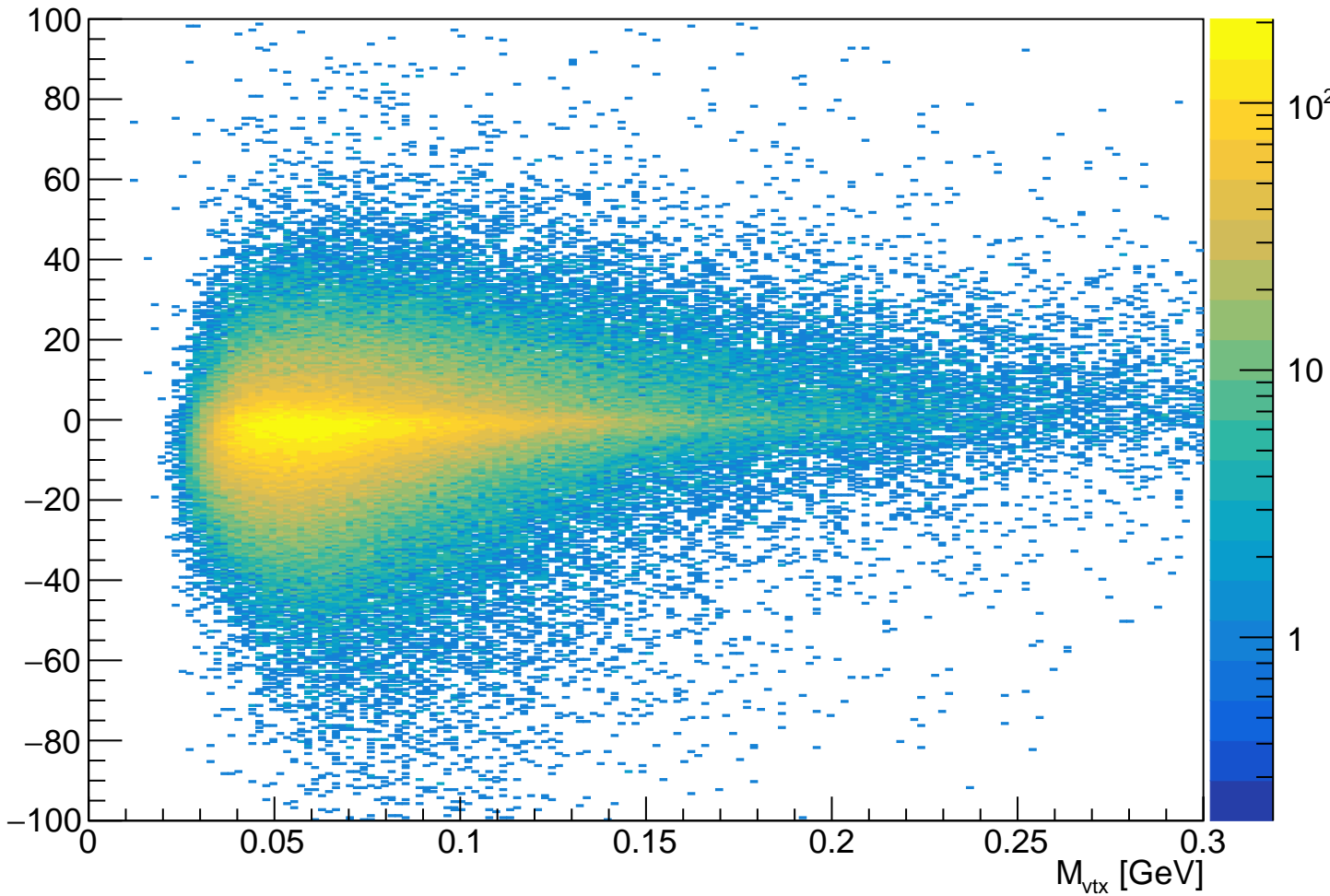
tridentNoInnerMatch-NoClusters_vtx_InvM_vtx_z_hh
