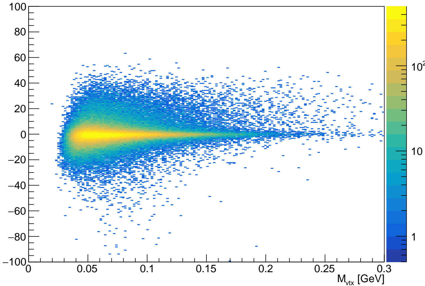
tridentL2L2-BothClusters_vtx_InvM_vtx_z_hh
