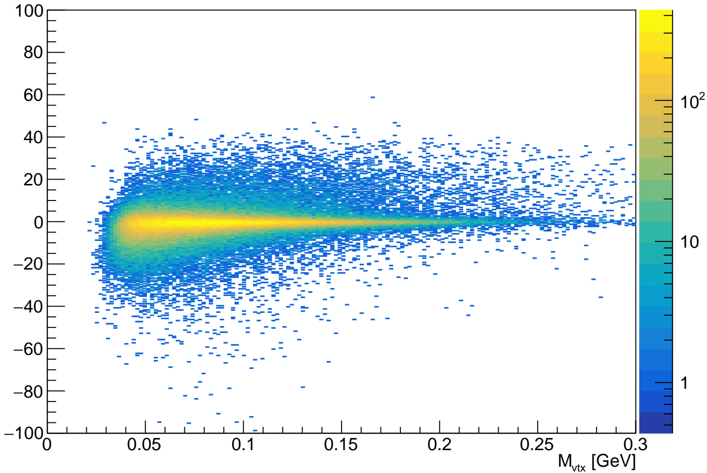
tridentL2L1-BothClusters_vtx_InvM_vtx_z_hh
