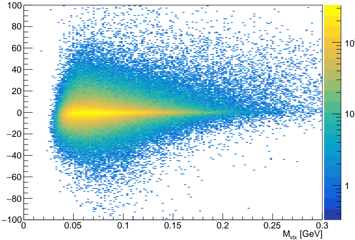
tridentNoInnerMatch-BothClusters_vtx_InvM_vtx_z_hh
