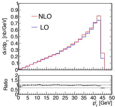
Sub-leading jet of e^+e^- \rightarrow w\bar{u}
