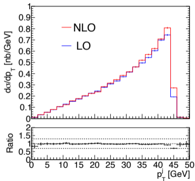
Leading jet of e^+e^- \rightarrow w\bar{u}
