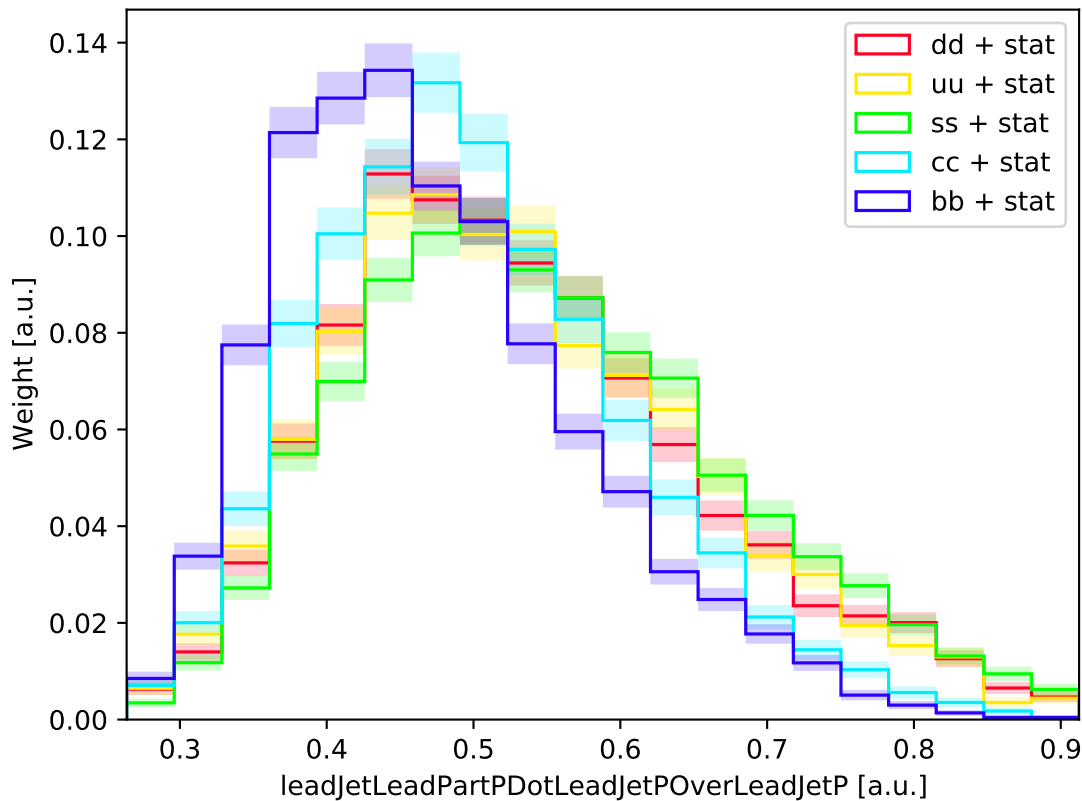
ILC-ILD : leadJetLeadPartPDotLeadJetPOverLeadJetP (normalized)
