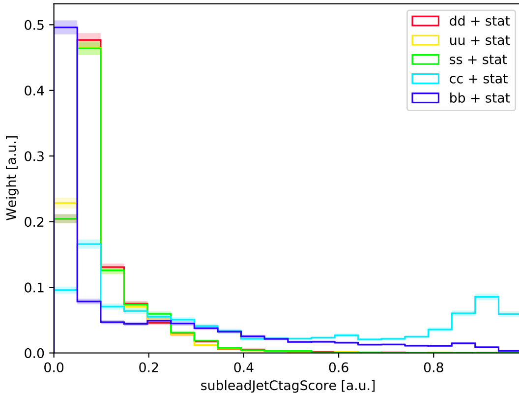
ILC-ILD : subleadJetCtagScore (normalized)
