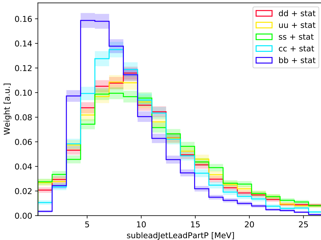
ILC-ILD : subleadJetLeadPartP (normalized)
