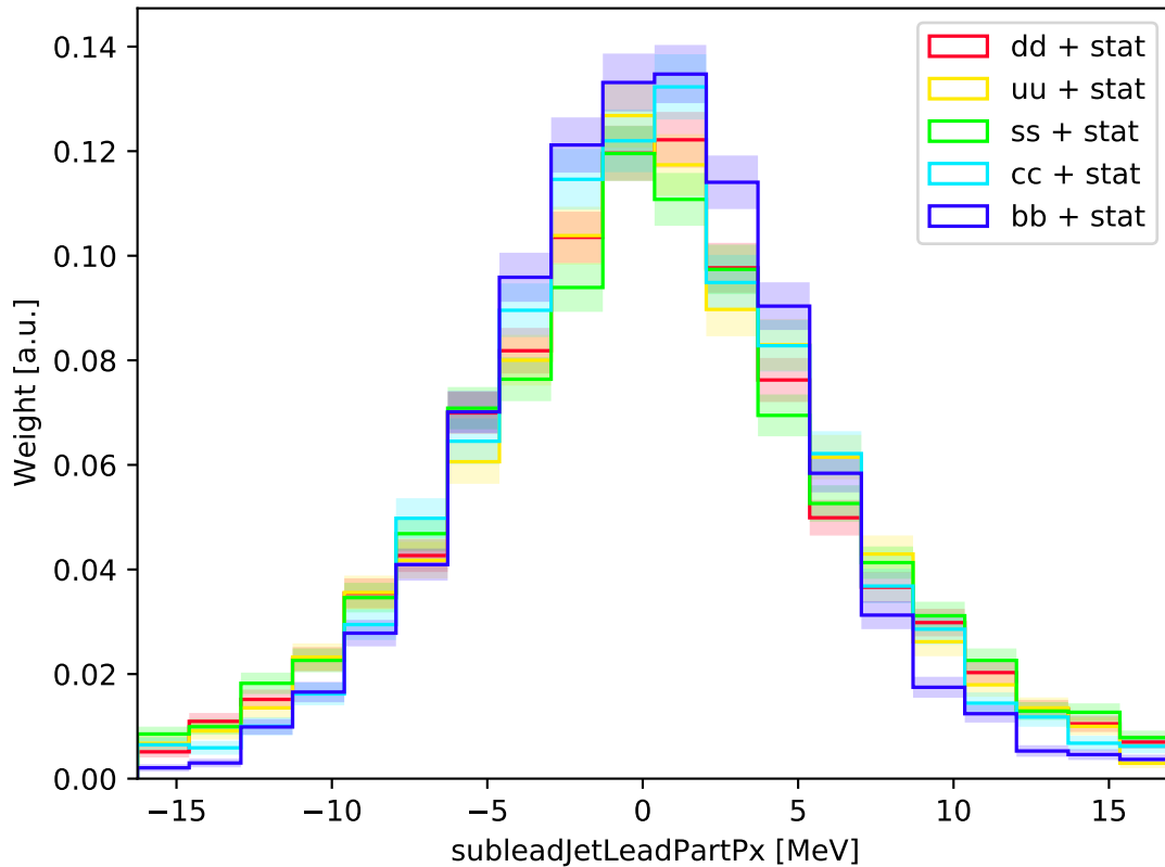
ILC-ILD : subleadJetLeadPartPx (normalized)
