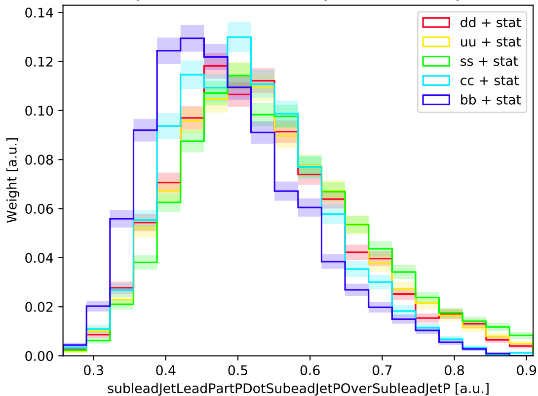
ILC-ILD : subleadJetLeadPartPDotSubeadJetPOverSubleadJetP (normalized)
