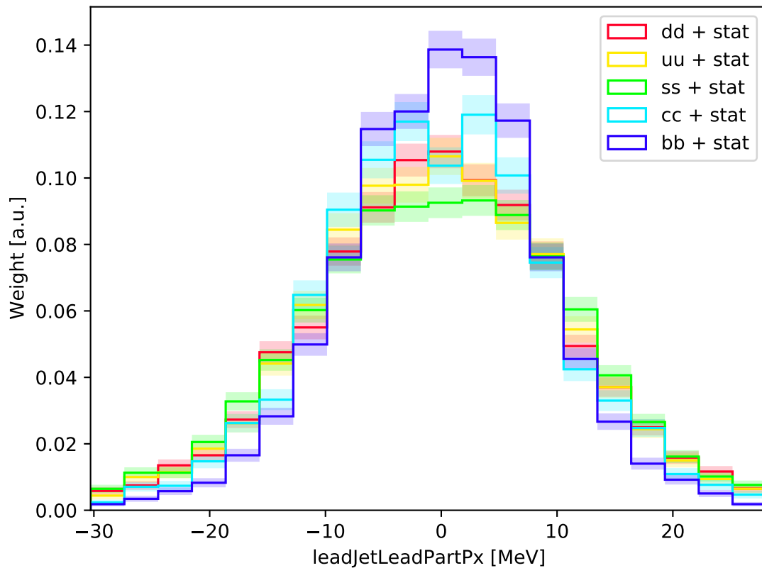
ILC-ILD : leadJetLeadPartPx (normalized)
