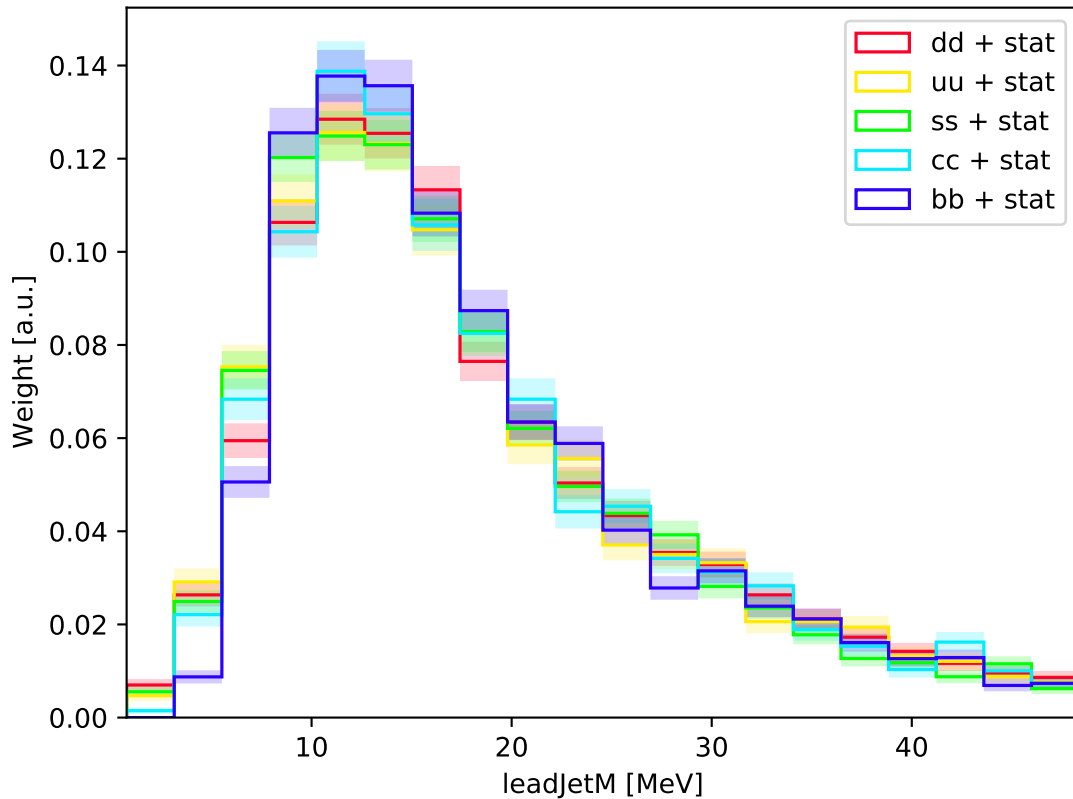
ILC-ILD : leadJetM (normalized)
