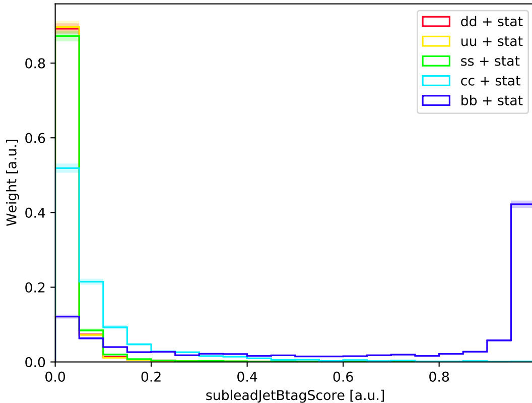
ILC-ILD : subleadJetBtagScore (normalized)
