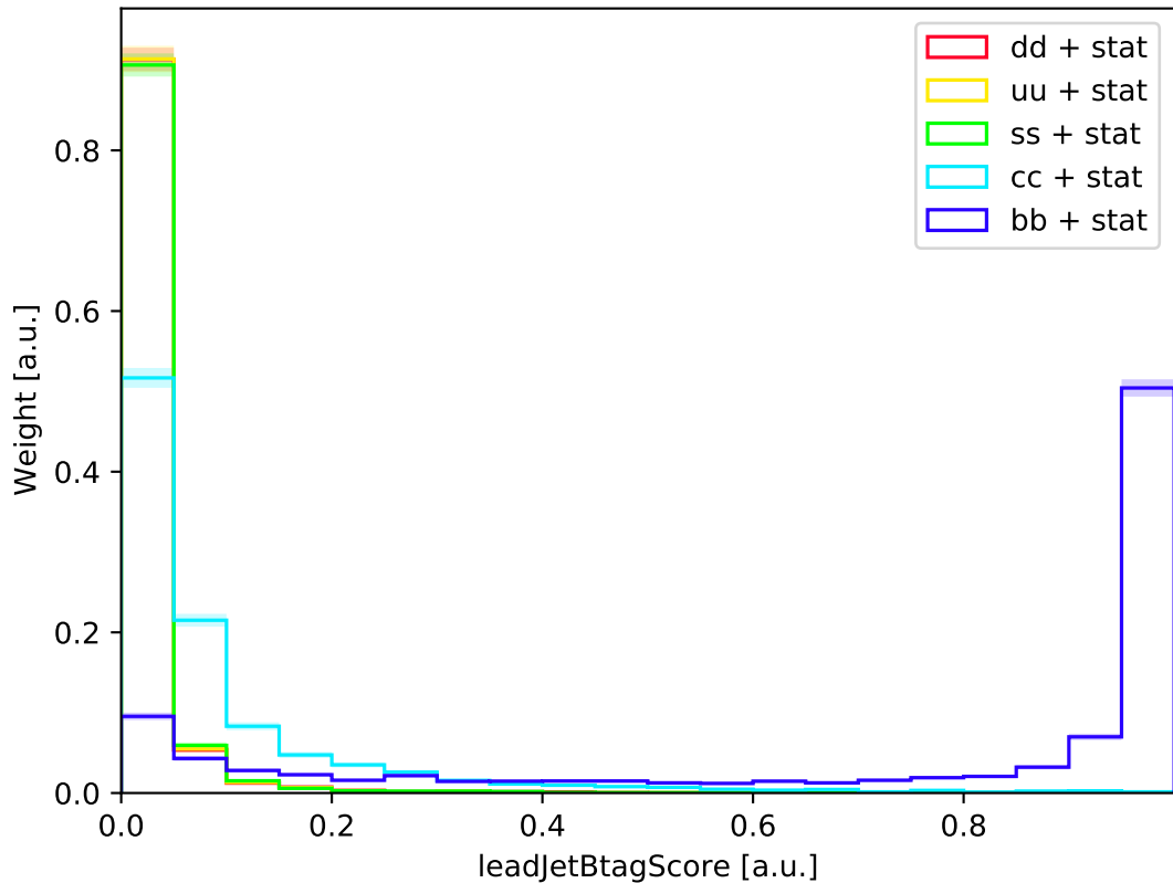
ILC-ILD : leadJetBtagScore (normalized)
