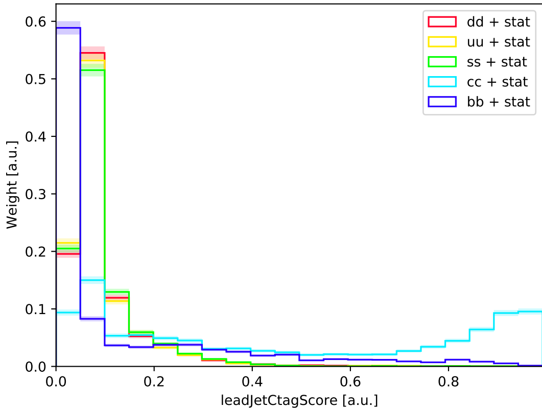
ILC-ILD : leadJetCtagScore (normalized)
