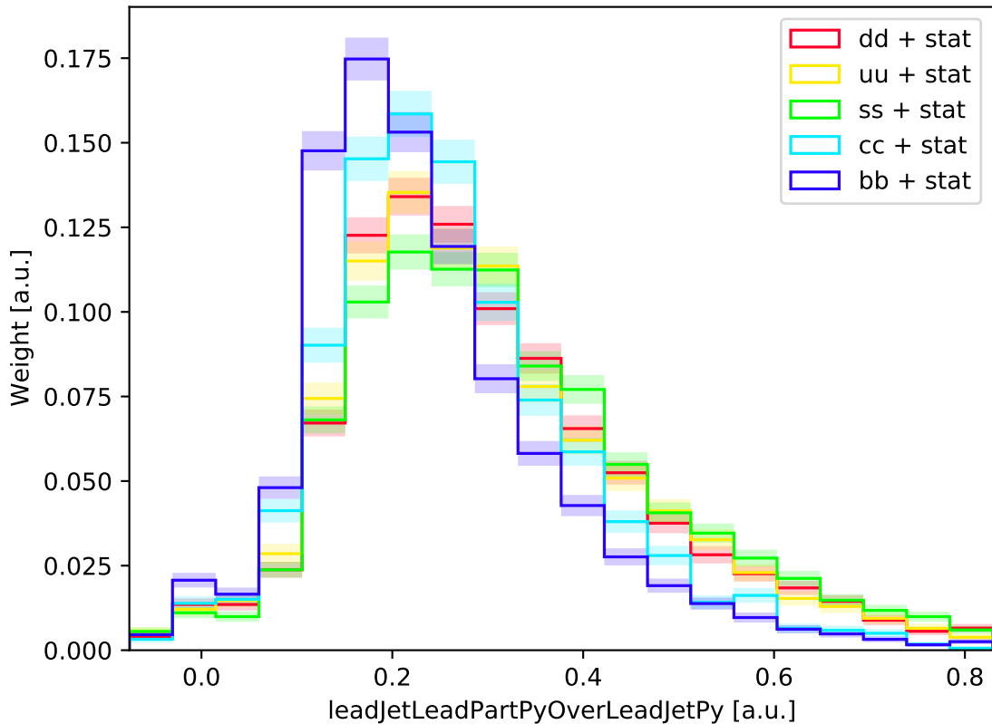
ILC-ILD : leadJetLeadPartPyOverLeadJetPy (normalized)
