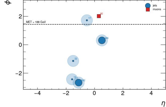
rank 7: AD score = 1527.632 (event 645641070) -- HLT objects
