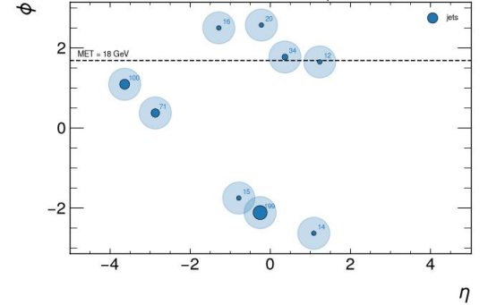
rank 2: AD score = 1407.460 (event 1672574499) -- HLT objects
