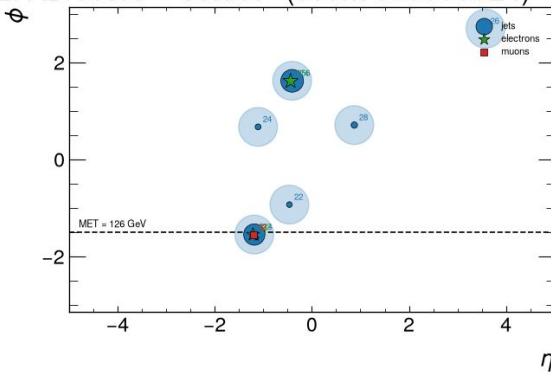
rank 152: AD score = 68.987 (event 359605924) -- HLT objects
