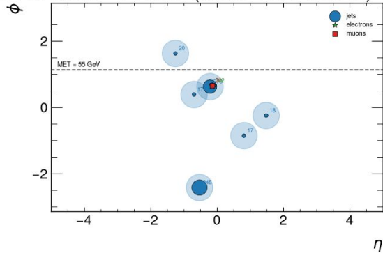
rank 146: AD score = 71.172 (event 1465697540) -- HLT objects
