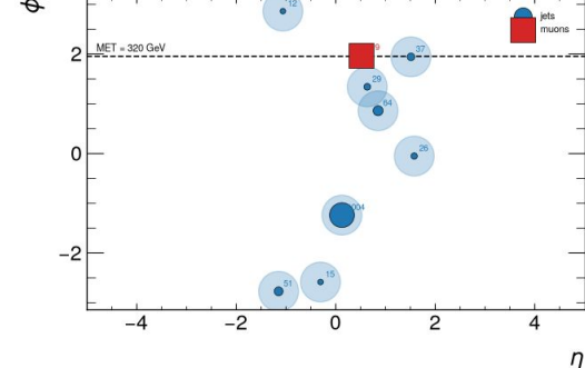
rank 2: AD score = 9828.545 (event 1653524401)
