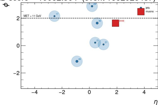
rank 1: AD score = 19082.504 (event 1852925487) -- HLT objects
