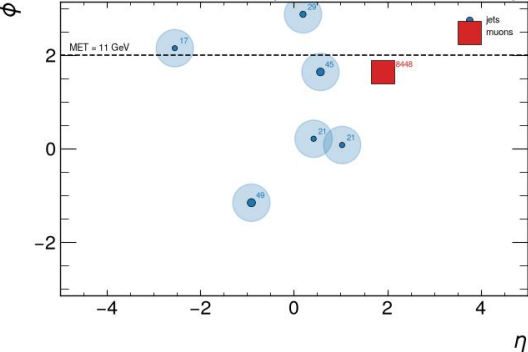
rank 1: AD score = 19082.504 (event 1852925487) -- HLT objects
