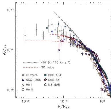
Figure: NFW Predictions vs. Observations(Oh et al. 2011)
