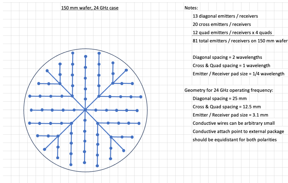
Figure 6a, Phased Array Layout Example for 150 mm Wafers
