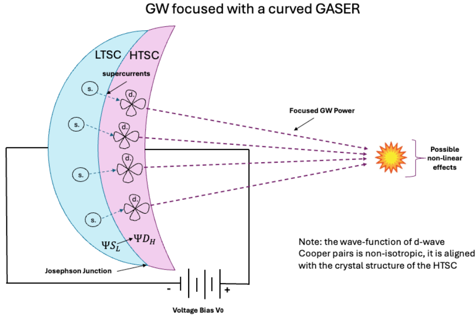
Figure 4, A curved GASER to create an HFGW focal point, adapted from [3], [7]
