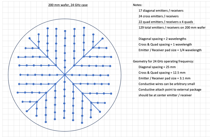
Figure 6b, Phased Array Layout Example for 200 mm Wafers
