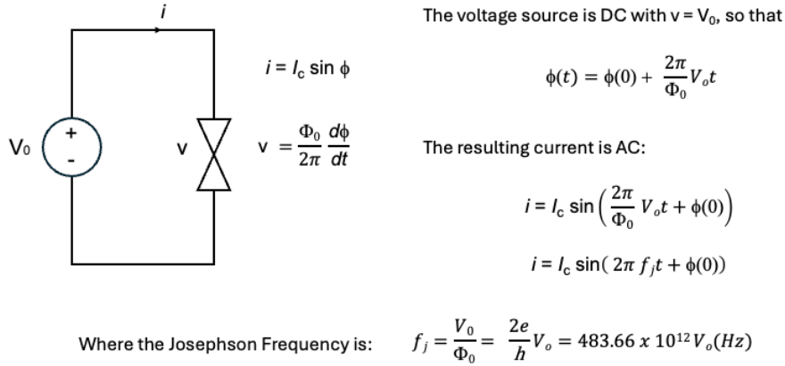
Figure 5, The AC Josephson Effect [9]
