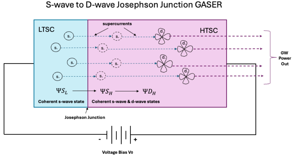
Figure 2, Graviton emissions at a s-wave to d-wave junction, adapted from [3]
